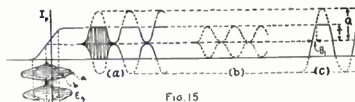
In This Undesirable Case the Smooth Undistorted Curve Produced by Reduction of the Impress Voltage is 73% as Effective as the Flat-Toppt One.
