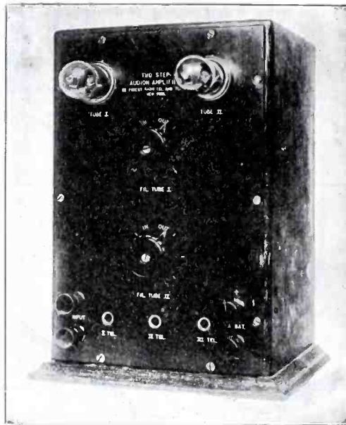
Fig. 20. A Typical Two-Stage Audion Amplifier.
