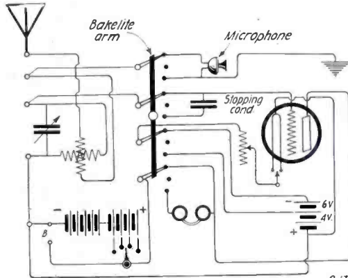
A Hook-Up for Utilizing the Same Vacuum Tube for Both Radiophone Transmission and Reception. A Switch Does the Trick.
