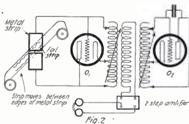
Fig. 2 A Circuit Ultra-Sensitive to Capacity Change.
