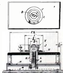
Constructional Details of Mr. F. B. Armstrong's Receiver, Showing How the Variable Condenser and the Little Detector are Made. The Four Arms Supporting the Primary Allows a Very Loose Coupling When Extended.
