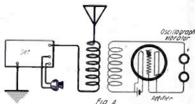
This Shows How the Oscillograph Vibrator Was Coupled to the Set During the Tests.
