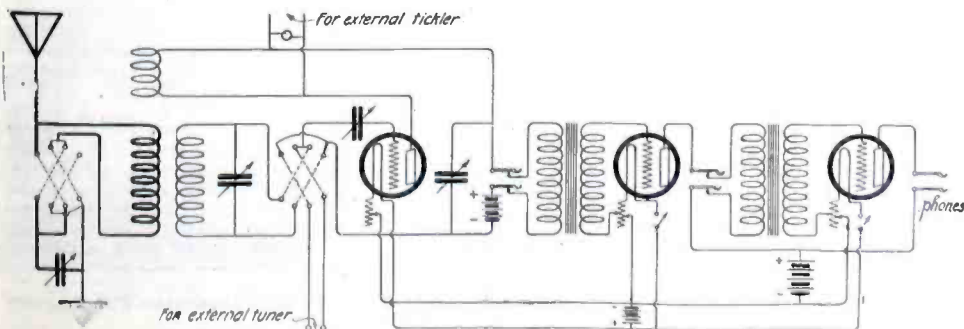
Schematic Circuit Diagram of the Hook-Up Used By Mr. Mathison in His Practical Sea-Going Receiver Which He Employs on Ship-board.
